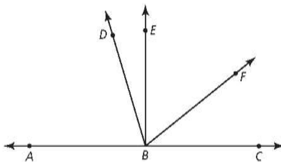
Non-Vertical Angles
