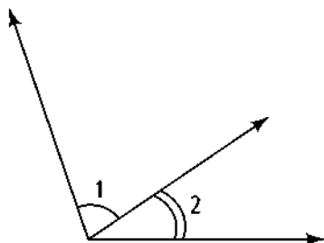
Adjacent Angles
